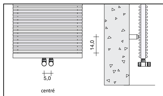
Schéma technique raccordement BA14D i5
