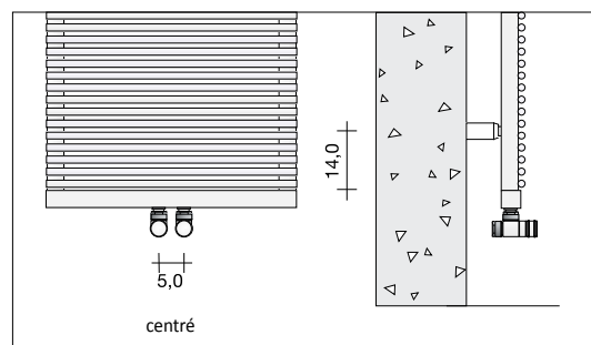
Schéma technique raccordement BA14 i5
